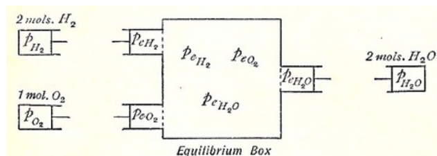
Figure: Maximum work of a gaseous reaction.
